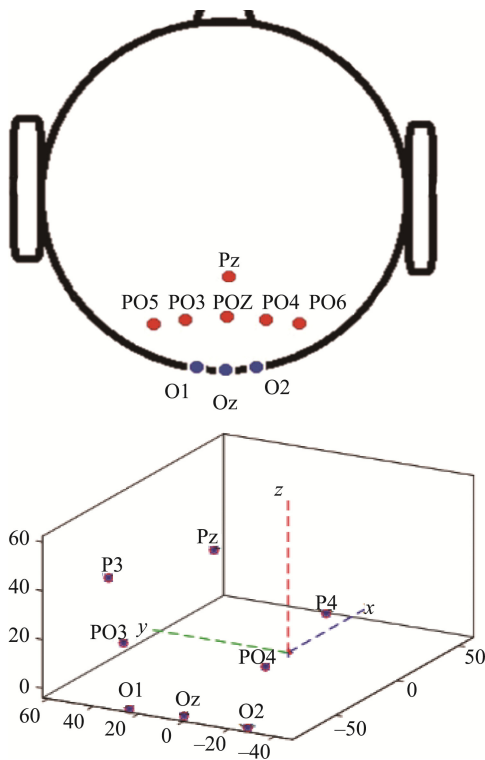
Fig.3 Electrode Channel Diagram
