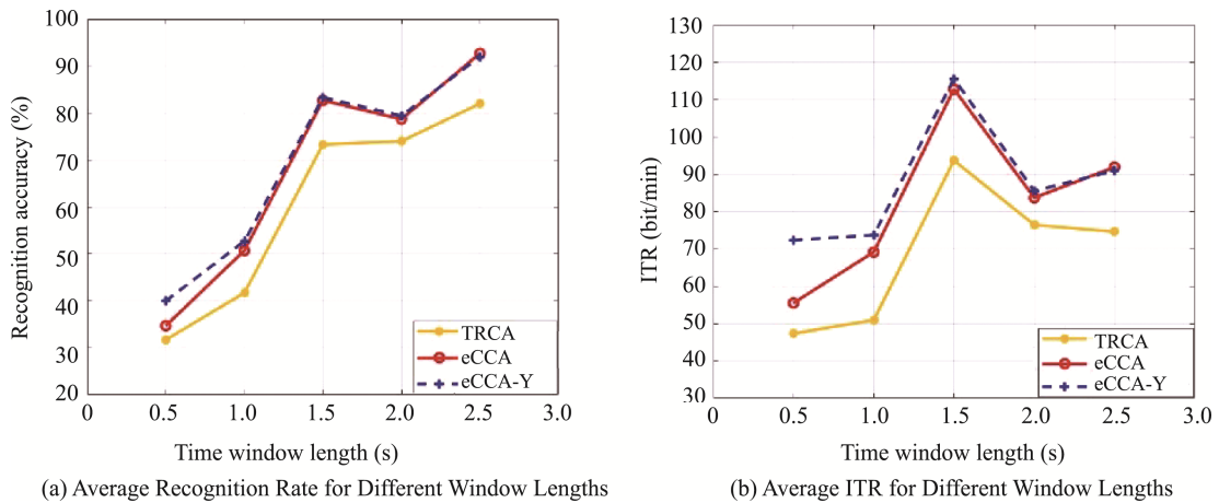
Fig.7 Performance of 3 Algorithms with Different Window Lengths
