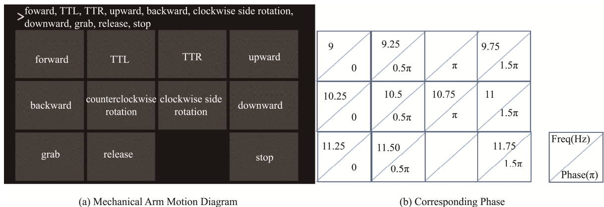
Fig.1 Mechanical Arm Excitation Model
