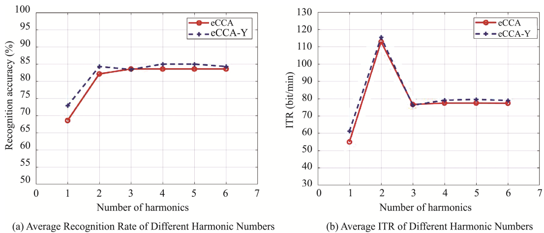
Fig.8 Algorithm Performance of Different Harmonic Orders
